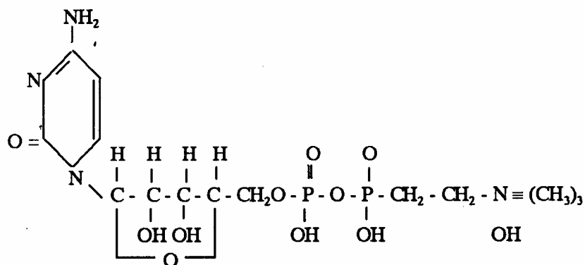
CDP-Cholin
