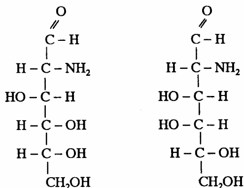
D - glucosamin
