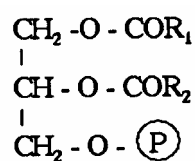
Acid phosphatidic
