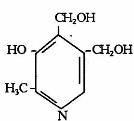
Pyridoxin
