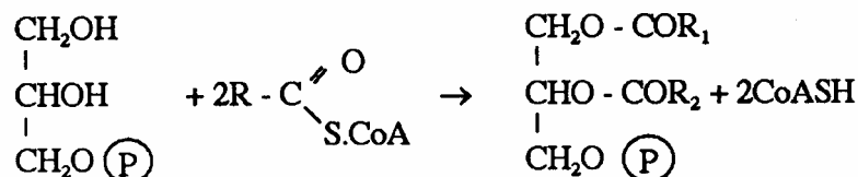
Glycerinphosphat
