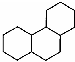
Perhydrophenantren
