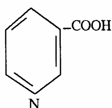
Acid nicotinic
