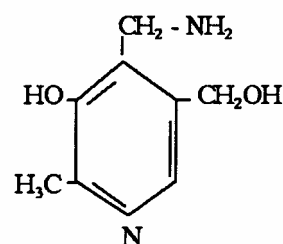
Pyridoxamin
